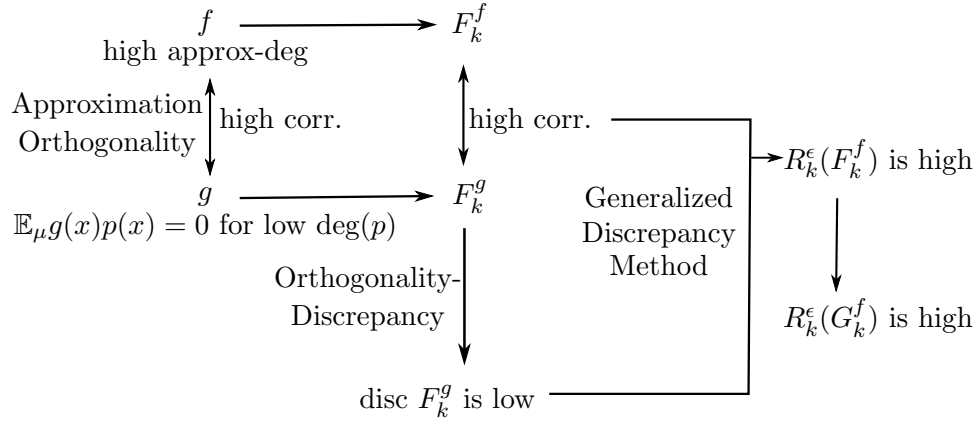
Figure 1: Proof outline
