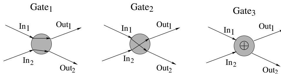
FIG. 3. Some gates of a well-structured circuit. Gates 1-2 are switching gates, and gate 3 sits in layer 0 and computes the parity (xor) function.
